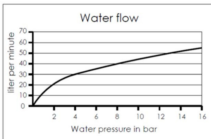
Flow-pressure diagram
